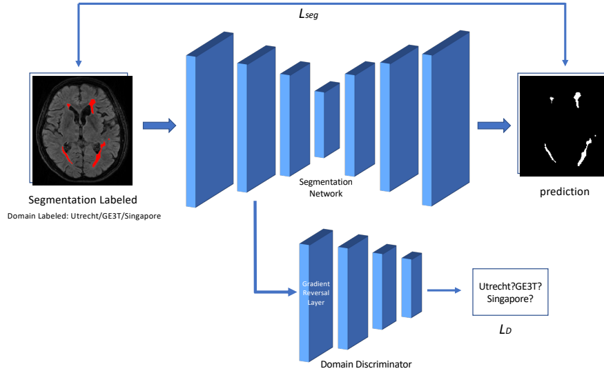
Fig. 1. Illustration of the proposed model which consists of a segmentation network and a domain discriminator
